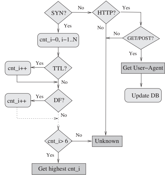
Figure 1: Classification algorithm.
